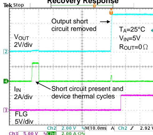
Short-Circuit to No-Load Recovery Response
