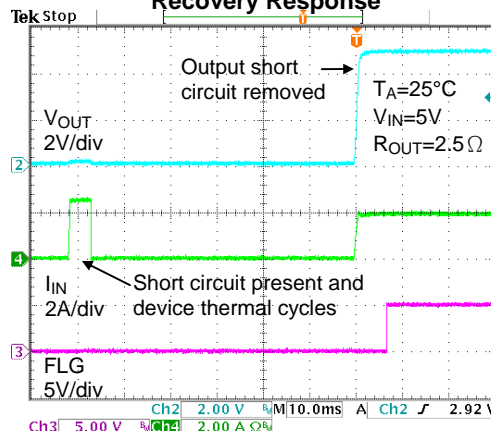
Short-Circuit to Full-Load Recovery Response
