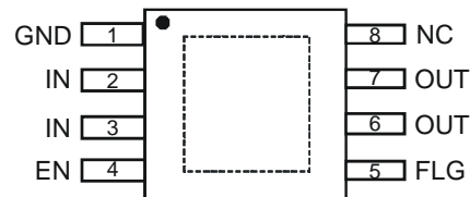
MSOP-8 /MSOP-8EP
